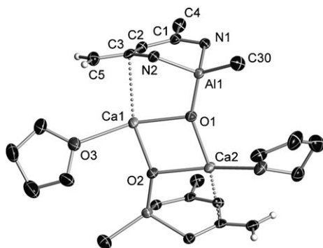
Figure 1. Core structure of [(L^1Al(Me)(\mu-O)Ca(thf))_2] ( 7 ); anisotropic displacement parameters are shown at the 50% probability level. Selected bond lengths [Å] and angles [°] of one half of a formula unit in the asymmetric unit: Al1–O1 1.740(2), Al1–N1 1.898(3), Al1–N2 1.900(3), Al1–C30 1.959(4), Ca1–O1 2.255(2), Ca1–O2 2.179(2), Ca1–O3 2.415(3), Ca1–C3 2.680(3), C3–C5 1.369(5); O1–Ca1–O2 82.47(9), O1–Al1–N2 104.24(12), N1–Al1–N2 98.14(13), Ca1–O1–Ca2 97.69(9), Ca1–O2–Ca2 97.26(9). Noncoordinating n -hexane molecules, substituents on the nitrogen atoms, and all hydrogen atoms (except those at C5 and C35) are omitted for clarity.
