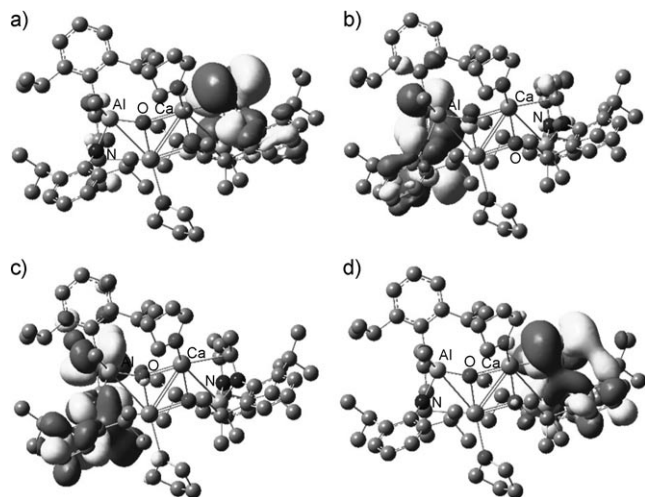
Figure 3. a) HOMO–1, b) HOMO, c) LUMO, and d) LUMO + 1 of 7 with energies –4.49, –4.48, –0.14, and –0.11 eV, respectively. All hydrogen atoms are omitted for clarity. The corresponding MOs of 8 are given in the Supporting Information.
